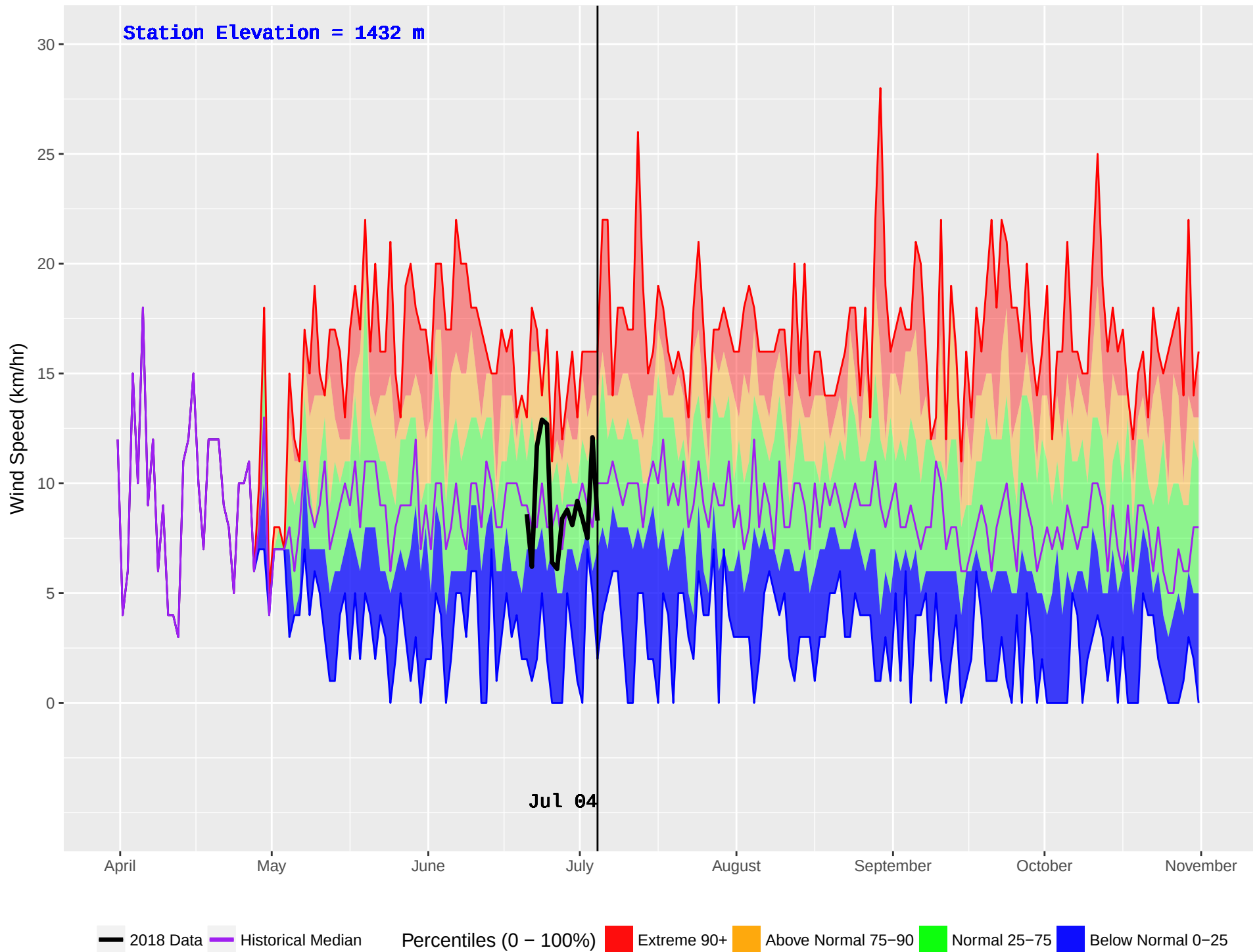
OCTOPUS CREEK (396) : Historical (2000–2016) and Current (2018) Noon Wind Speed
